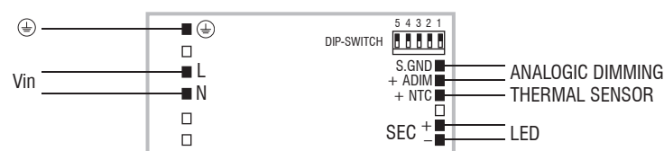
ADIM diagram - Collegamento ADIM
